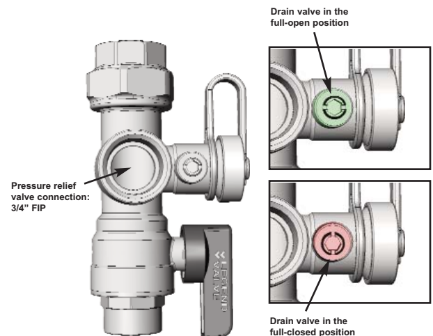
Drawing B: Hot Water Isolation Valve
