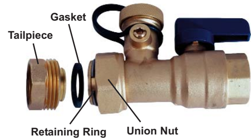
Photo A: Cold Water Isolation Valve
